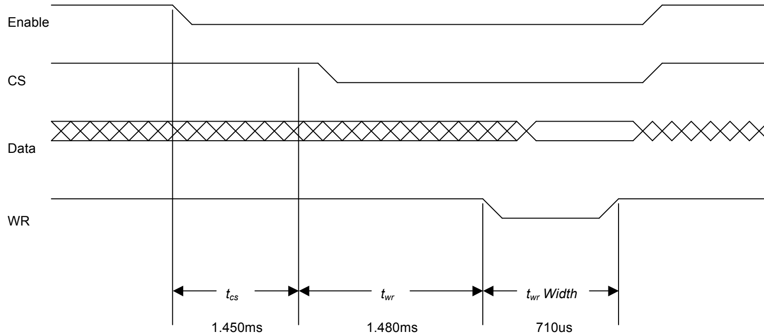
Figure 1: Slow Device Write Cycle
