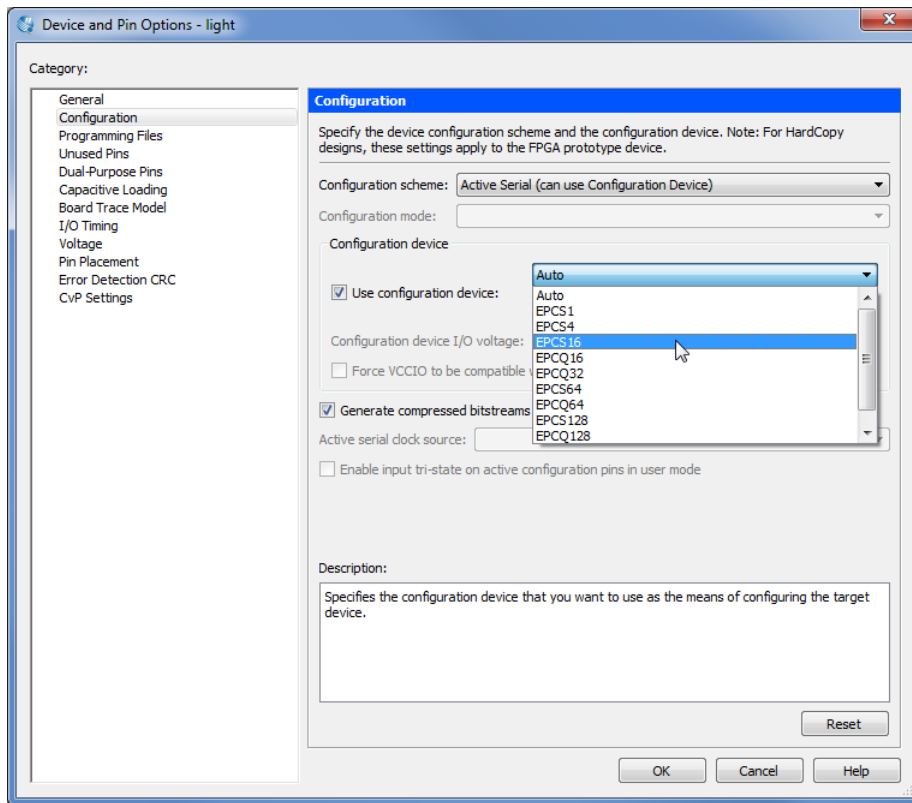
Figure 45. Specifying the configuration device.
