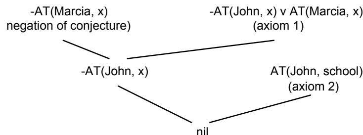
Figure 3-1. Refutation Tree for example problem.
